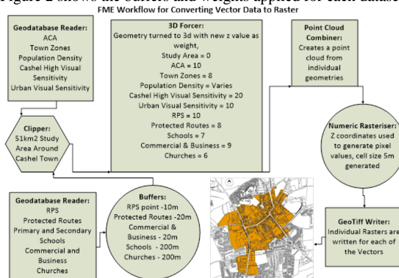
Figure 2 FME workflow for generating weighted raster maps.
