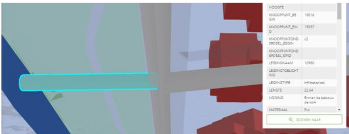
Figure 5. Open sewage locations data with additional attributes about the material, form, width etc.
