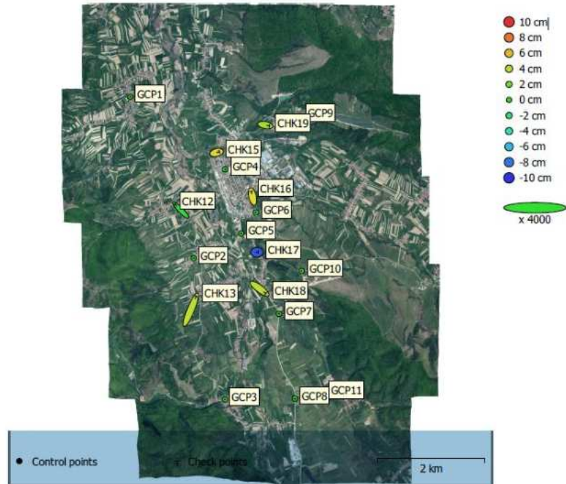
Figure 2 - The designed flight block for the town of Ştei. Disposition of GCP and CHK.
