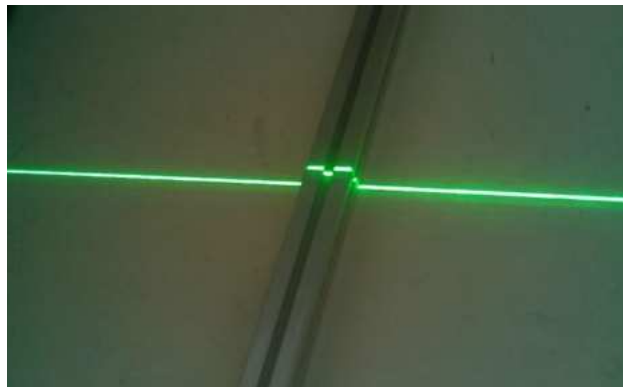
Figure 9: Image acquisition of projected laser line for triangulation-based creation of a point cloud
